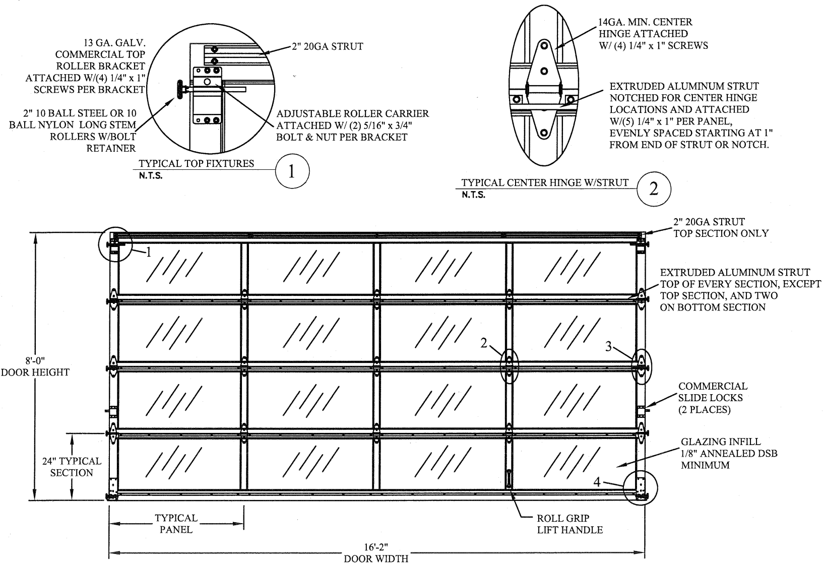
DOOR INTERIOR ELEVATION
